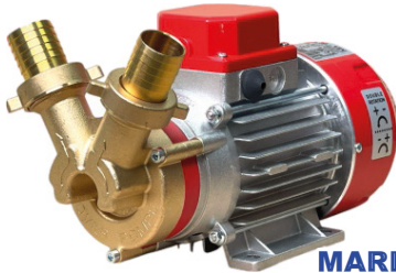
MARINA 30
