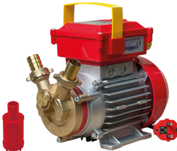
ROVER 20 By-Pass
